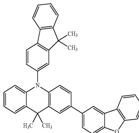
(Compound 5)
