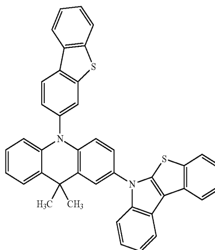
[Chemical Formula 6]
