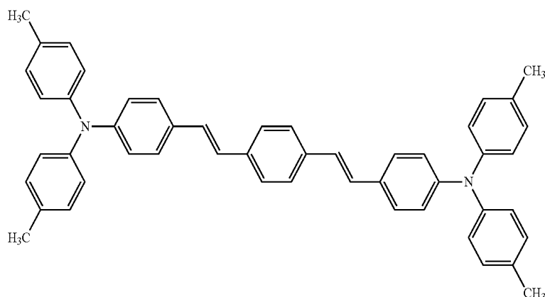
[Chemical Formula 88]
