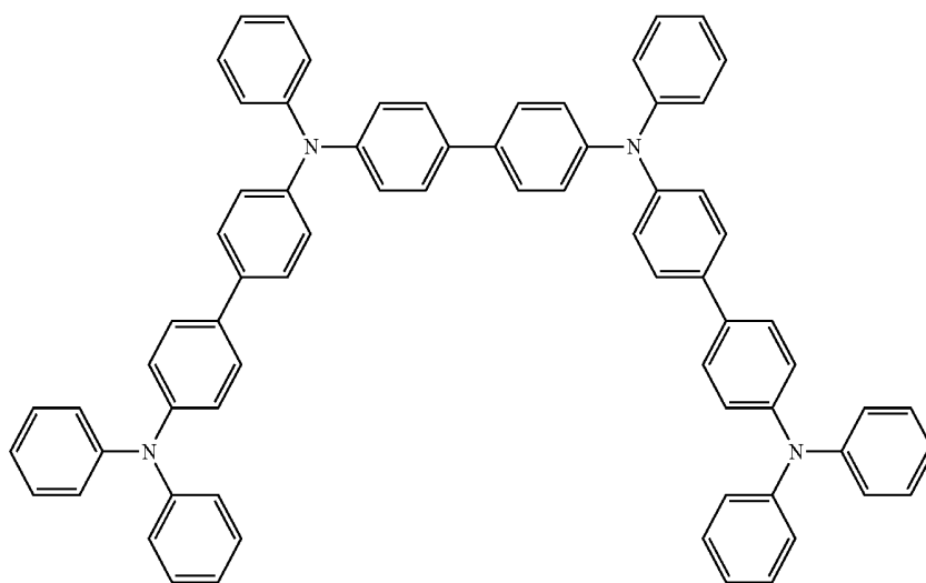
[Chemical Formula 87]
