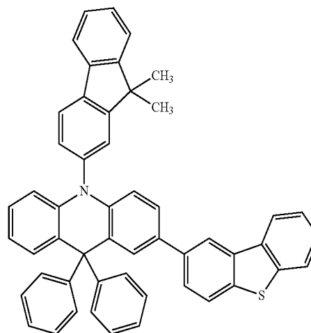
[Chemical Formula 7]
