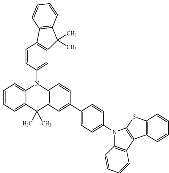
(Compound 49)
