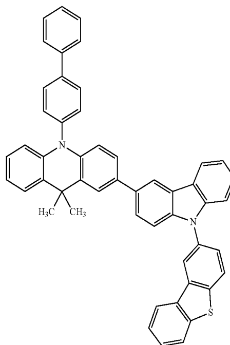
(Compound 51)
