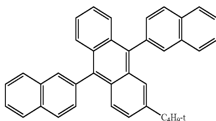
[Chemical Formula 88]
