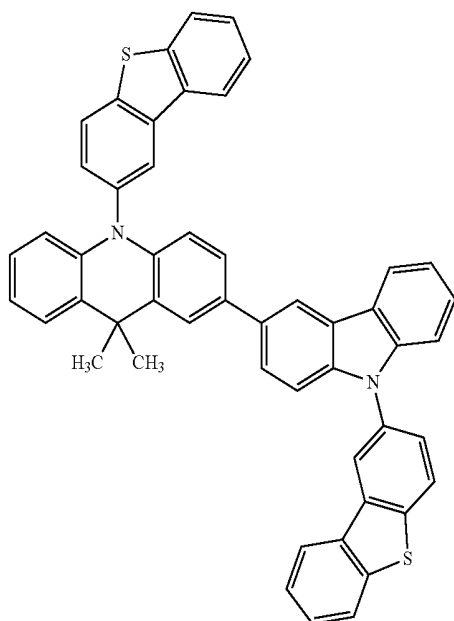
(Compound 50)
