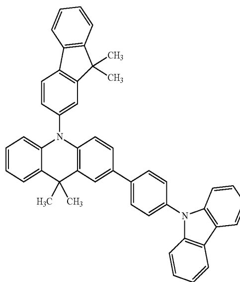
(Compound 52)
